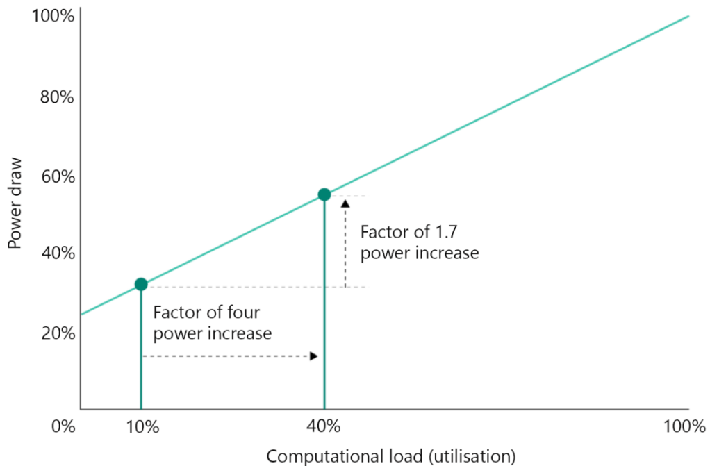
Figure 6: As utilisation increases, power per computational output decreases.
