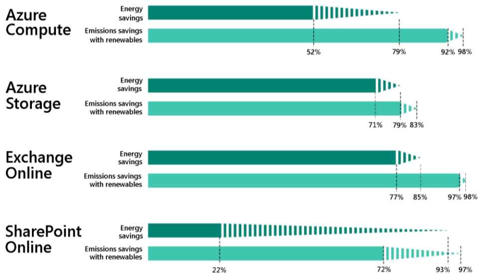
Figure 4: The range of energy and emissions savings by cloud service. 'Energy savings' shows the energy savings of the data centre electricity used in Microsoft Cloud services over the on-premises equivalents. 'Emissions savings (with renewables)' shows the emissions savings of the Microsoft Cloud services over the on-premises equivalents, taking into account the purchase of zero-emission renewable electricity to power the Microsoft Cloud.
